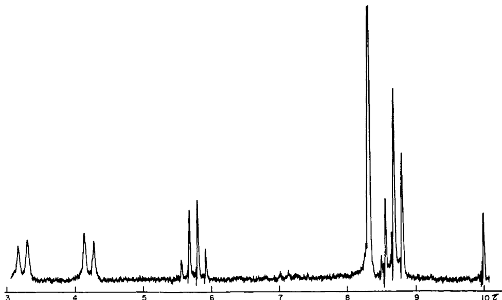
Figure 1. Nmr spectrum, 60 MHz, 1-carbethoxy-4-isopropylidene-1,4-dihydropyridine, 40° in carbon tetrachloride.
