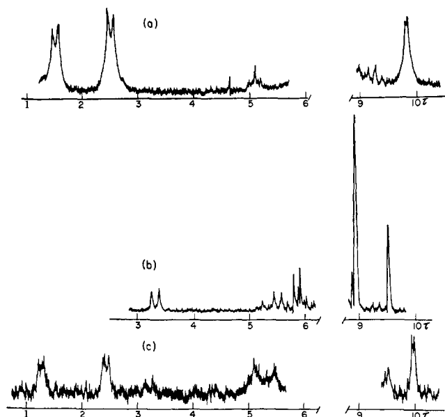
Figure 2. Nmr spectra, 60 MHz, 40°: (a) 2-(4-pyridyl)-2-methylpropylmagnesium chloride, 1.0 M in THF; (b) result of treating Grignard reagent in a with ethyl chloroformate; (c) result of treating 1-carbethoxy-4,4-(1,1-dimethylspirocyclopropyl)-1,4-dihydropyridine with butylmagnesium bromide.
